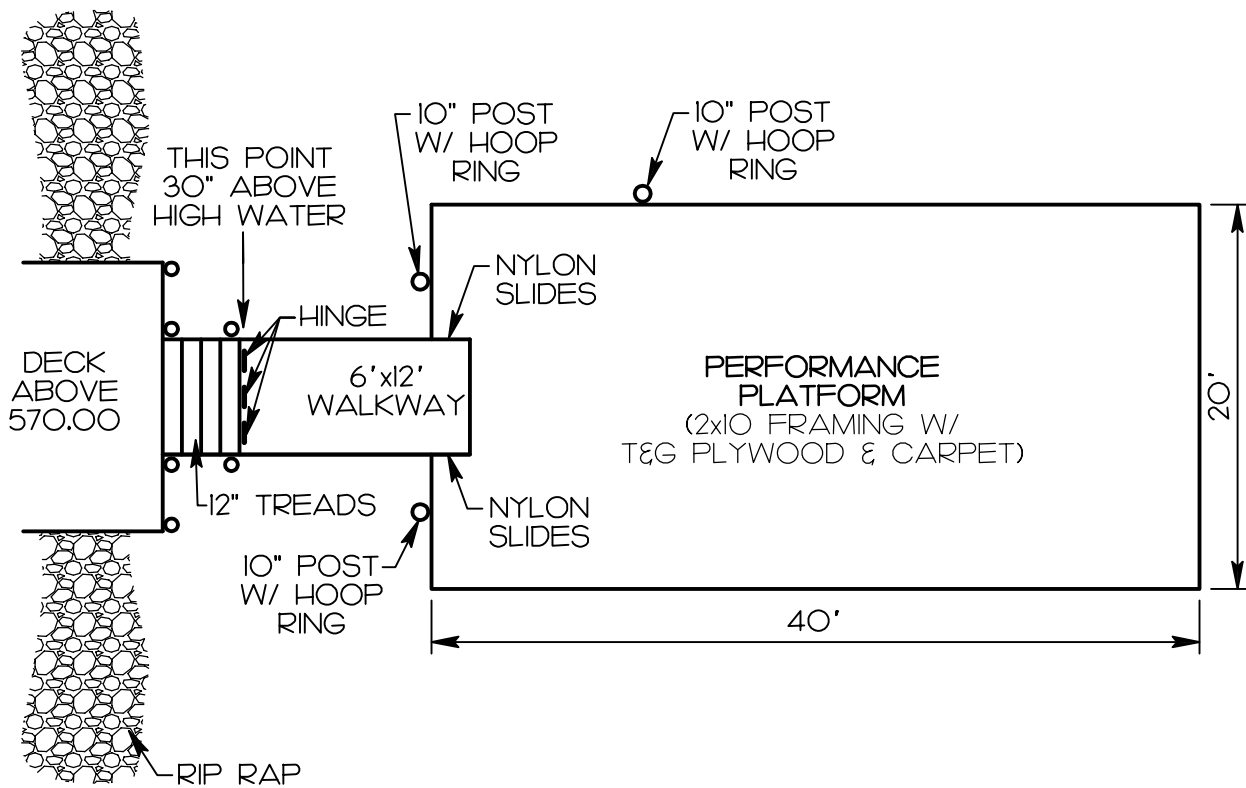
LAYOUT
